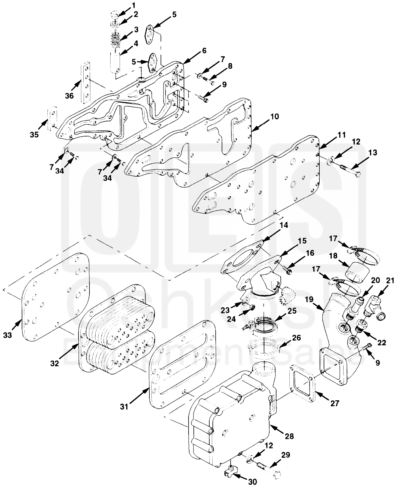
Figure 18. Oil Cooler
